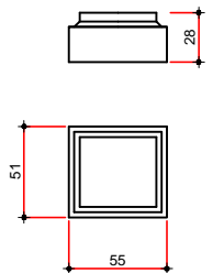
BASE (B-2) Esc. 1/20
